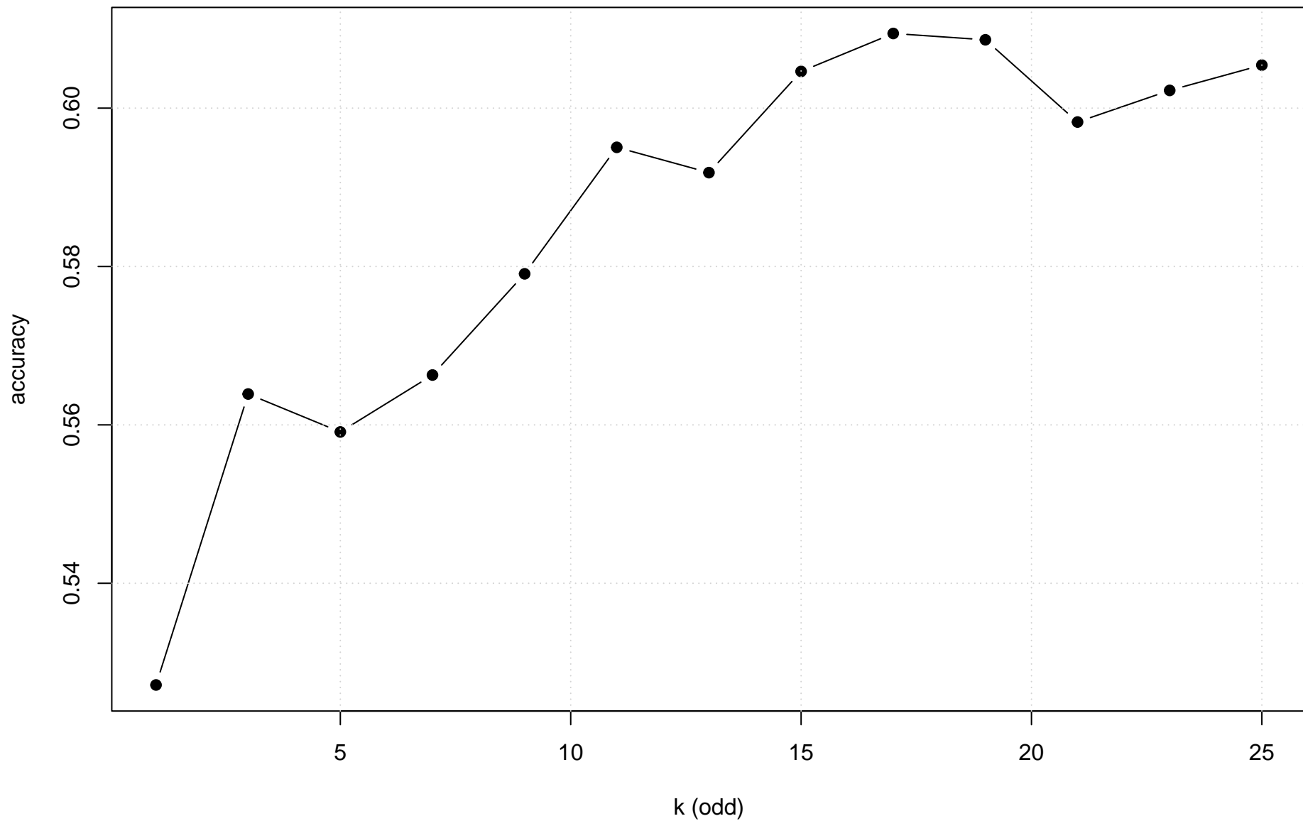
k-NN accuracy (chosen subset: small )
