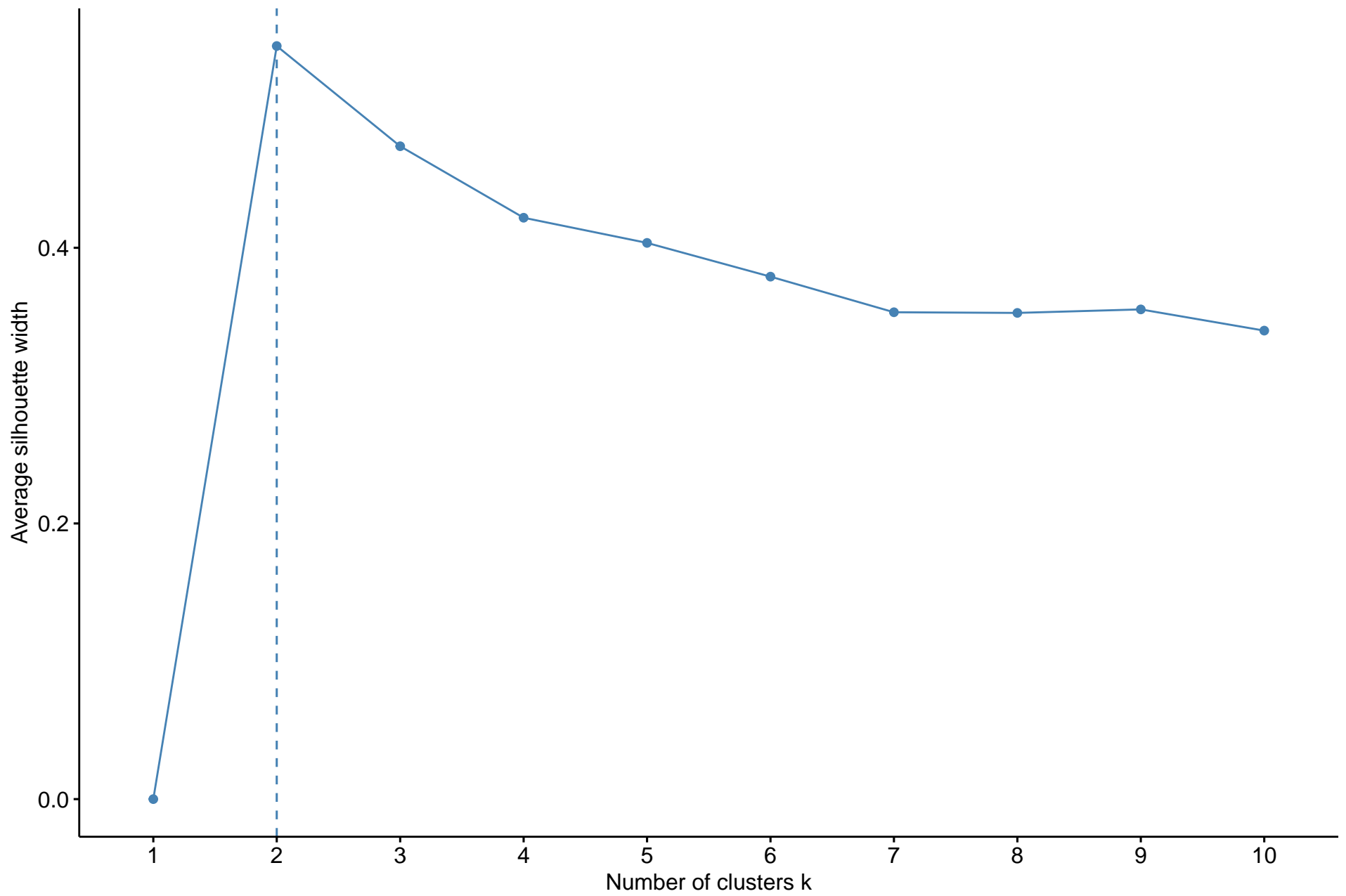
fviz_nbclust: silhouette (kmeans)
